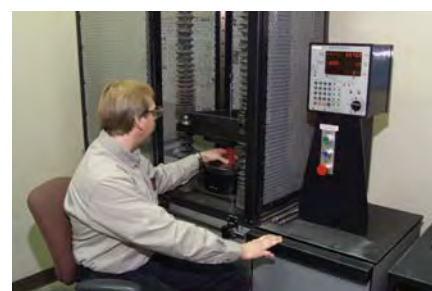
Computer Controlled Spring Testing - Utilizing custom software, spring testers track and verify consistency in spring dimensions and rates.
